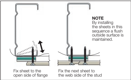
FIGURE 4 SCREW FASTENING
