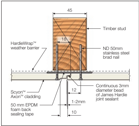
FIGURE 10 BRAD NAIL FIXING
