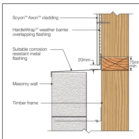
FIGURE 26 HORIZONTAL JUNCTION 2
