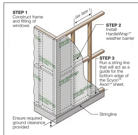
FIGURE 2 PREPARATION
