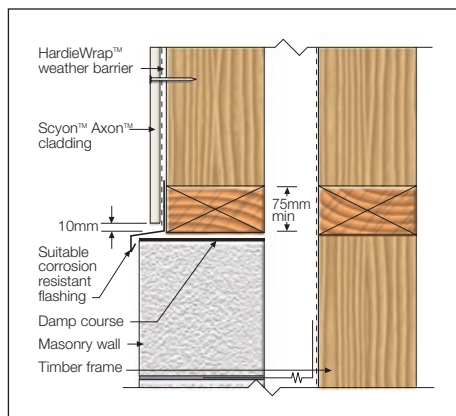
FIGURE 25 HORIZONTAL JUNCTION 1
