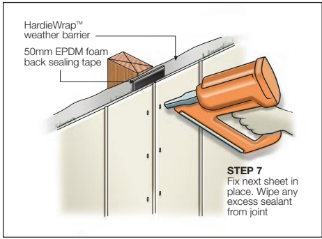
FIGURE 9 FIX NEXT SHEET
