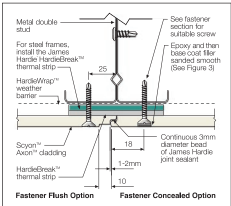
FIGURE 12 SHEET JOINT ON STEEL: FLUSH AND CONCEALED FIXING OPTIONS
